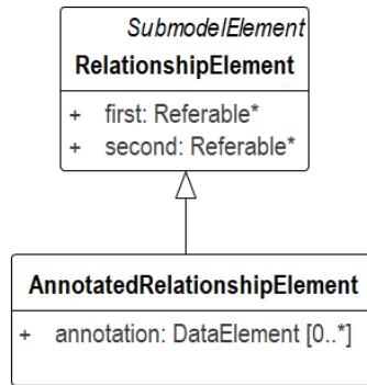
Figure 33 Metamodel for Relationship and Annotated Relationship Elements
