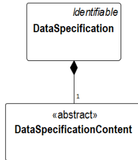
Figure 43 Concept of Data Specification Templates
