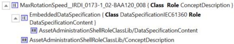
Figure 114 Example Embedded Data Specification IEC61360 of Concept Description for Property “MaxRotationSpeed”
