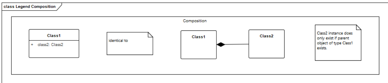
Figure 135 Composition in Metamodel in UML - Legend
