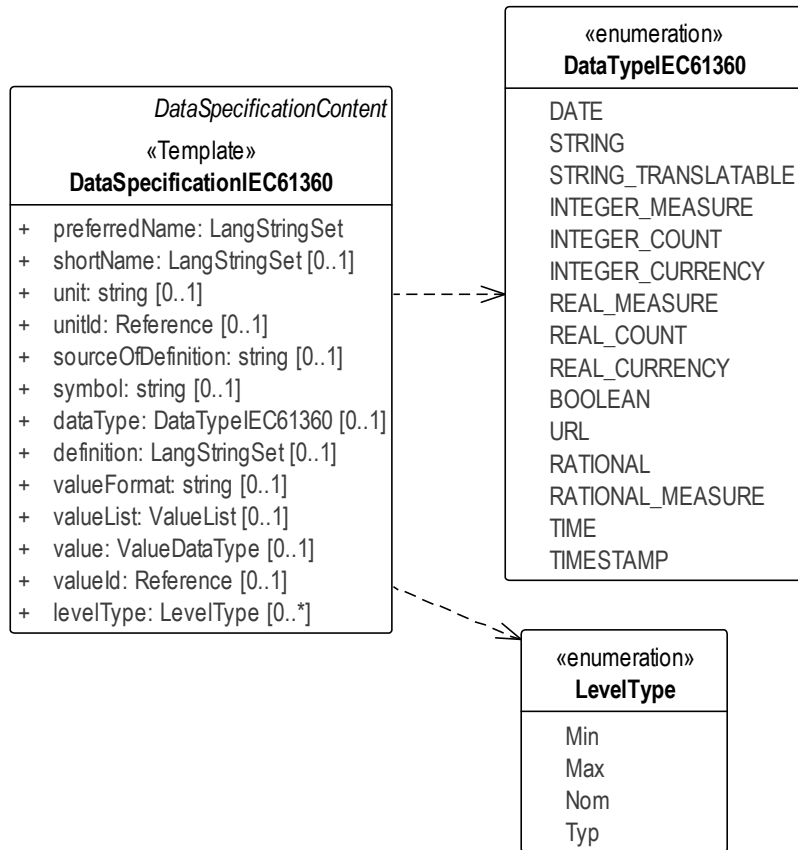
Figure 44 Data Specification Template for defining Property Descriptions conformant to IEC 61360
