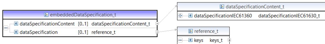
Figure 61 Data specification via IEC 61360 property attributes
