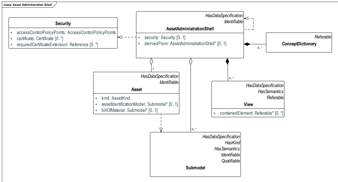
Figure 22 Metamodel AssetAdministrationShell
